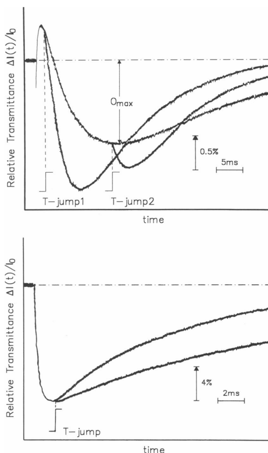
FIGURE 1 Experimental kinetic curves of formation and decay of O_{640} ( a ) (top) and decay of M_{410} ( b ) (bottom) intermediates of the bR photocycle. The unperturbed kinetic is combined with relaxation curves after T-jump(s). An accelerated decay kinetic of the M_{410} intermediate ( b ) shows the absolute amplitude of the T-jump. Initial temperature 10^\circ\text{C} ( \tau_{1/2} = 17 \pm 1 \text{ ms} ). The amplitude of the T-jump is 7.5 \pm 0.7^\circ\text{C} ( \tau_{1/2} = 7 \pm 0.5 \text{ ms} ).
